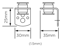
Gypframe GAH1 Acoustic Hanger
