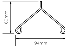
Gypframe GAH2 Acoustic Hanger
